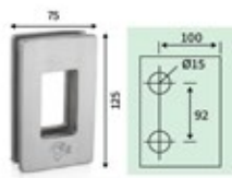
R1-SGH-012 Rectangle Sliding Handle (5x3) Satin ₹ 1400/-
