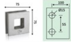
R1-SGH-013 Square Sliding Handle (3x3) Satin ₹ 1100/-
