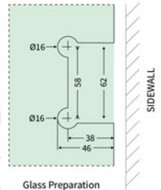
R1-BSH-08 Fix Hing for Wall to Glass Fix Panel
