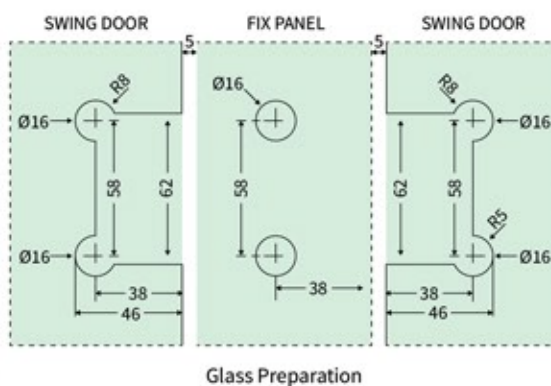
R1-BSH-07 Glass to Glass Hinges for Two Door (T-Hinges)
