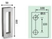
R1-SGH-011 Rectangle Sliding Handle (6x2) Satin ₹ 1300/-
