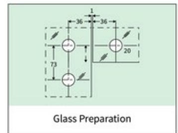
R1-PF-606 (Small L)
